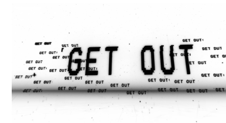
Corrupted Stellarium
